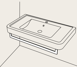
portasciugamani frontale frontal towel-rail 83 x 8 x 3,5h OPPSF100 104 x 8 x 3,5h OPPSF120
