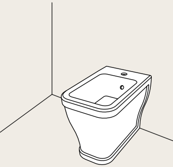
installazione a terra back to wall installation 57 x 36 x h44 OPVAQ
