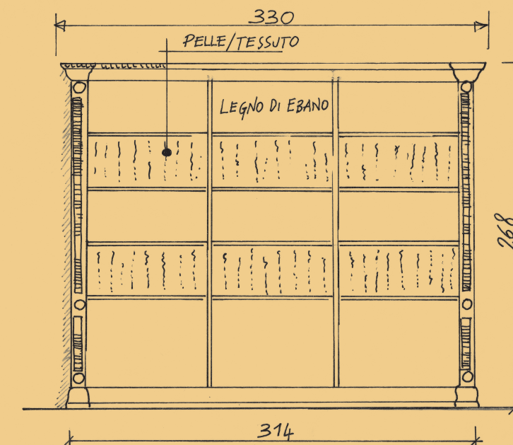
Cucina MAJESTIC – PROGETTARE LA BOISERIE MAJESTIC kitchen – DESIGN OF THE BOISERIE
