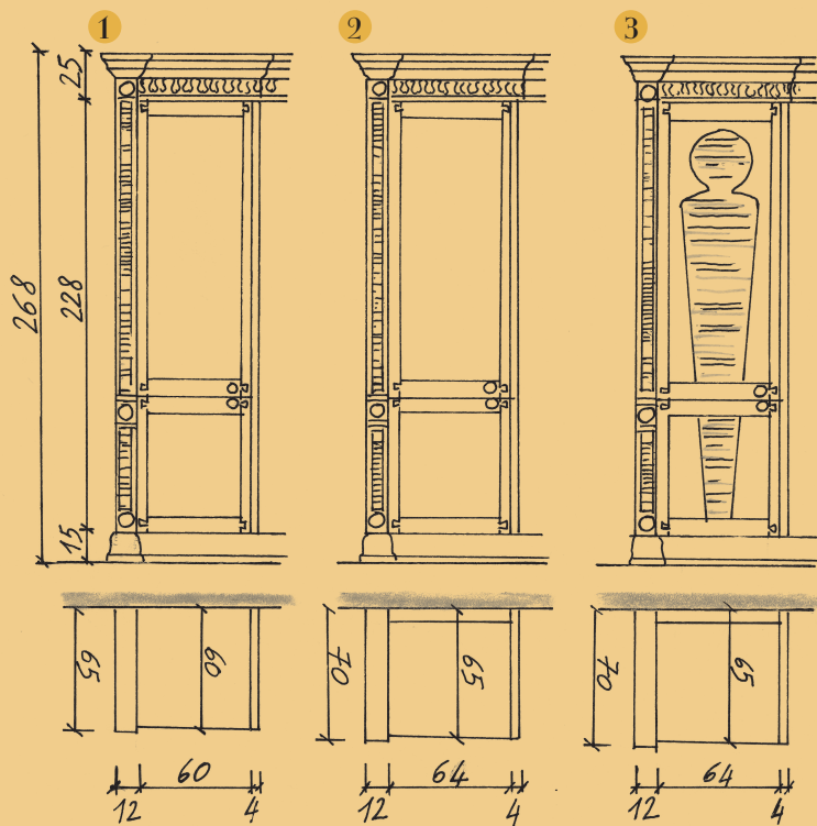
Cucina MAJESTIC – TIPOLOGIA COLONNE MAJESTIC kitchen – COLUMNS TYPOLOGY
