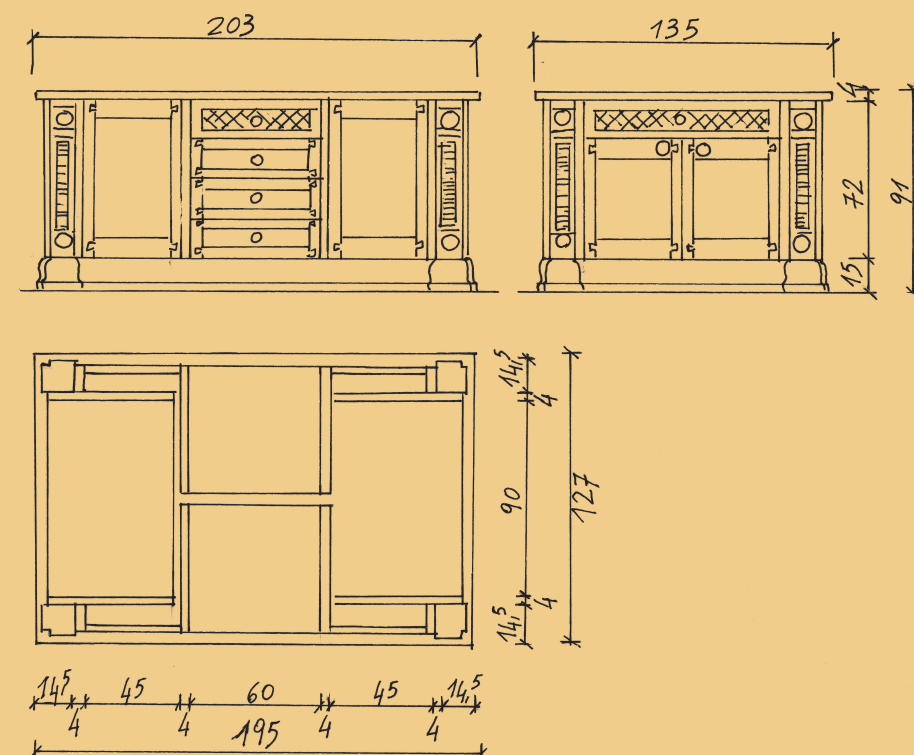
Cucina MAJESTIC – PROGETTARE L'ISOLA MAJESTIC kitchen – DESIGN OF THE ISLAND BENCH
