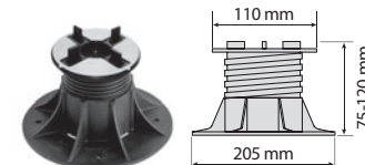
201004 V150 Supporto regolabile autolivellante Adjustable paving support self leveling head mm 75/120
